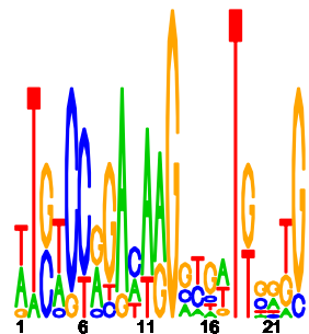
upstream meme PSSM #2; e=19
