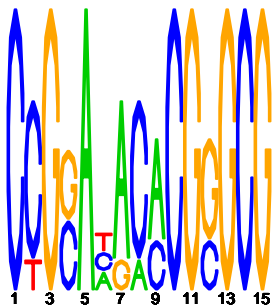
upstream meme PSSM #1; e=14
