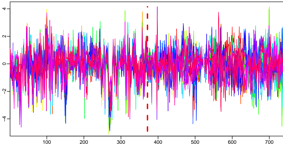
upstream meme PSSM #1; e=14
