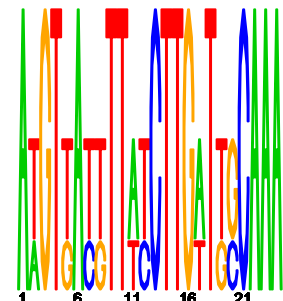
upstream meme PSSM #2; e=1.8
