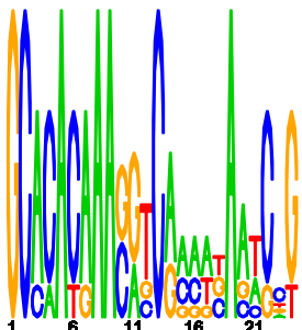
upstream meme PSSM #1; e=0.12
