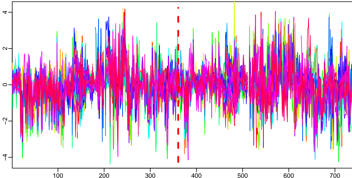
upstream meme PSSM #1; e=0.12
